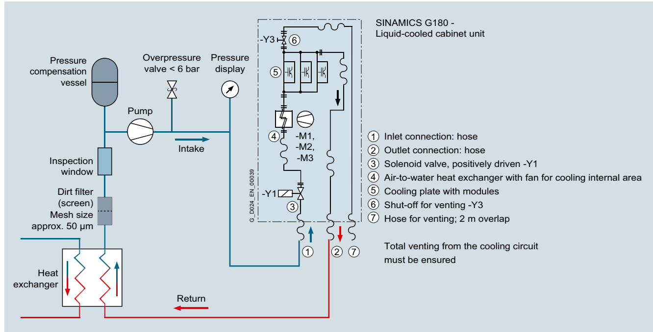
SINAMICS G180 liquid-cooled cabinet unit – recommended layout for a closed cooling circuit
